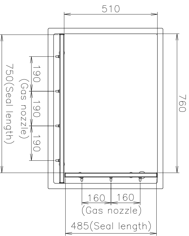
Chamber detail
